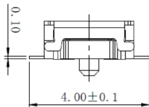
REFERENCE DRAWING
